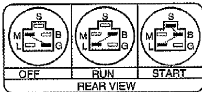
IGNITION SWITCH
