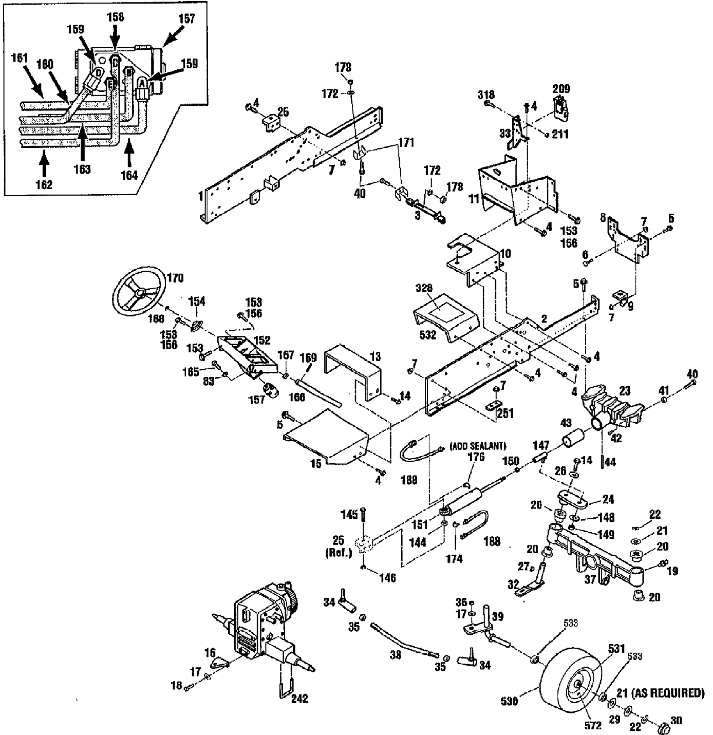
FRAME AND STEERING ASSEMBLY
