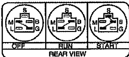
IGNITION SWITCH
