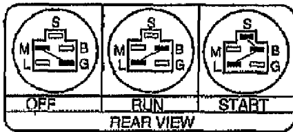
IGNITION SWITCH
