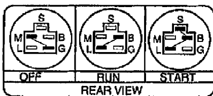
IGNITION SWITCH
