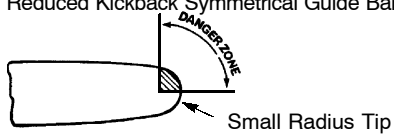
Symmetrical Guide Bar
