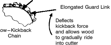
Contoured Depth Gauge
