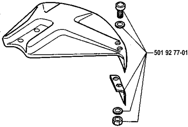
Guard, compl. 502 10 47-01
