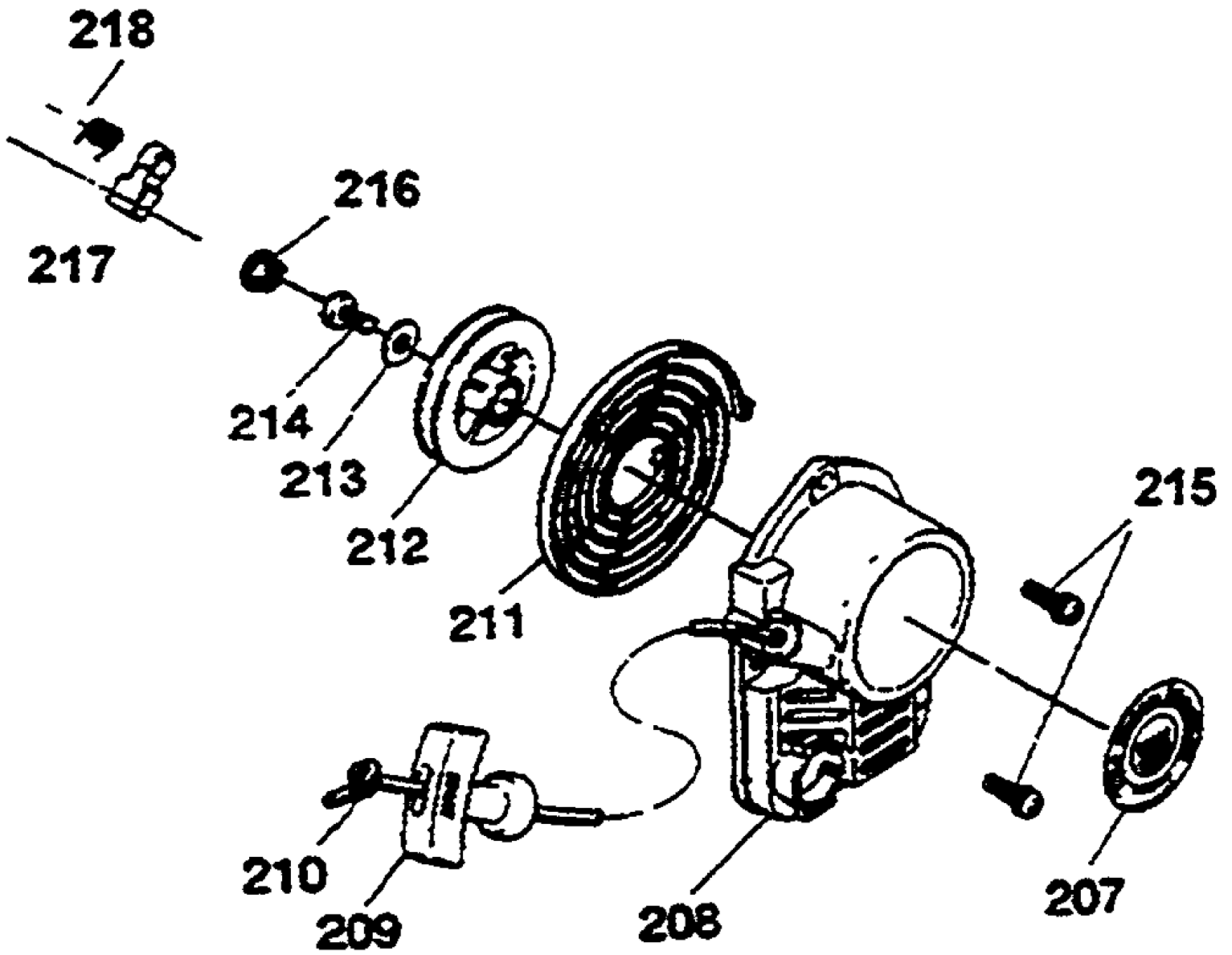
206 — STARTER ASSY
