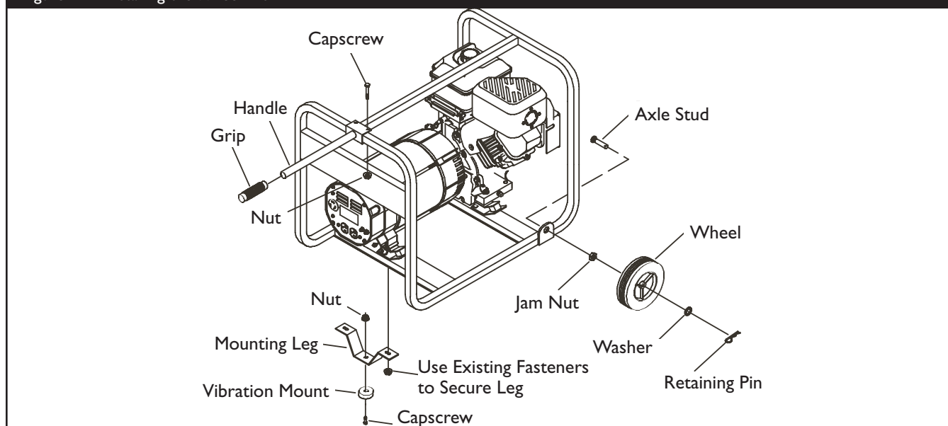
Figure 2 — Installing the Wheel Kit
