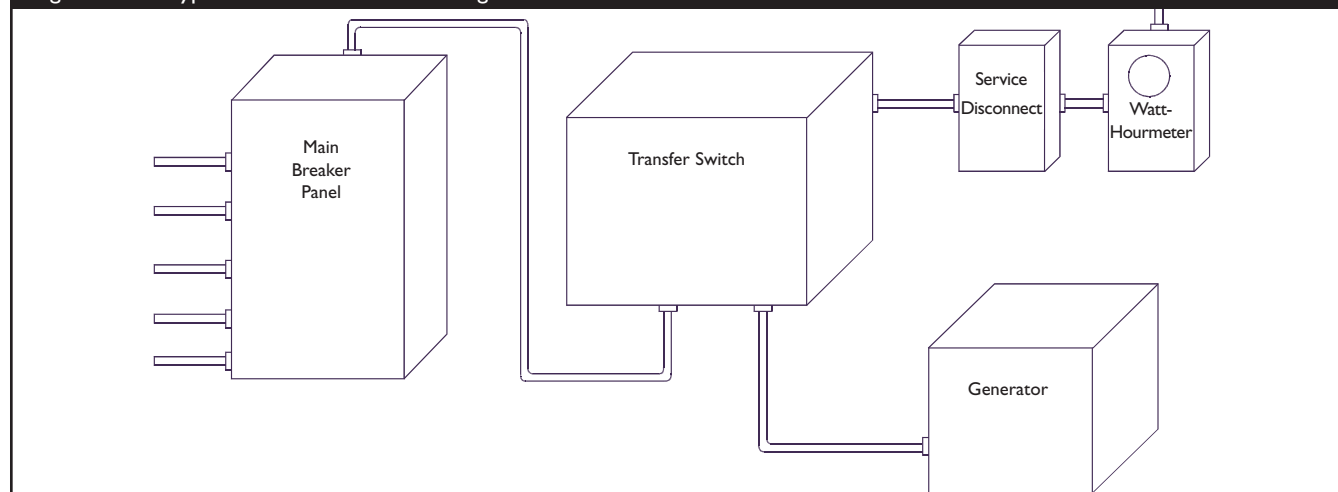
Figure 2 — A Typical Transfer Switch Mounting
