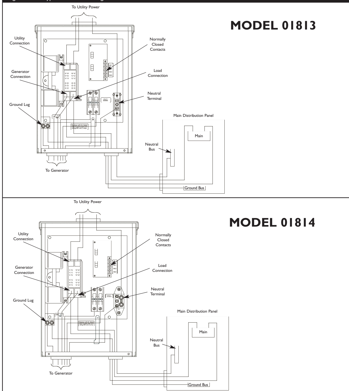
Figure 3 — A Typical Installation Diagram for Transfer Switch
