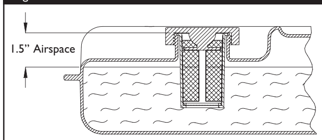
Figure 3 — Fuel Level
