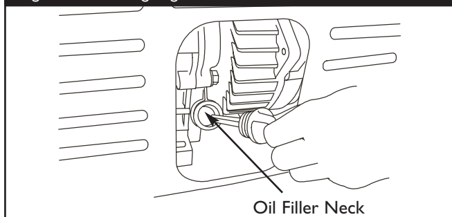
Figure 2 — Adding Engine Oil
