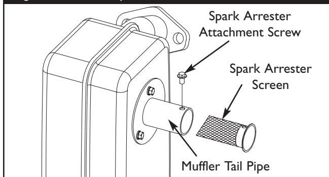
Figure 16 — Service Spark Arrester Screen
