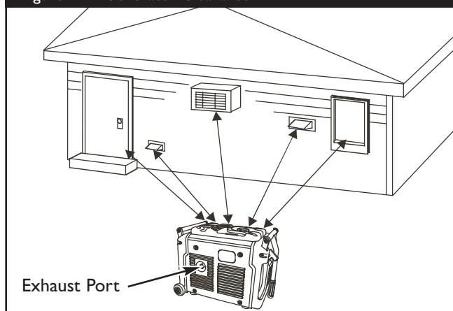
Figure 4 — Generator Clearance
