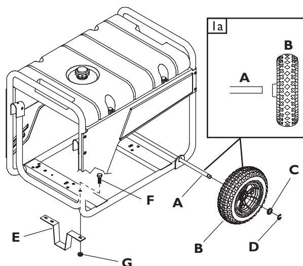
Figure 1 — Install Wheel Kit
