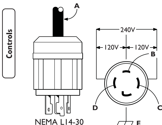
Figure 4 — 120/240 Volt AC, 30 Amp Receptacle
