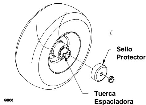
FIGURE 4 ENSAMBLE RUEDA DELANTERA
