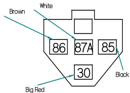
Seat Relay Connector
