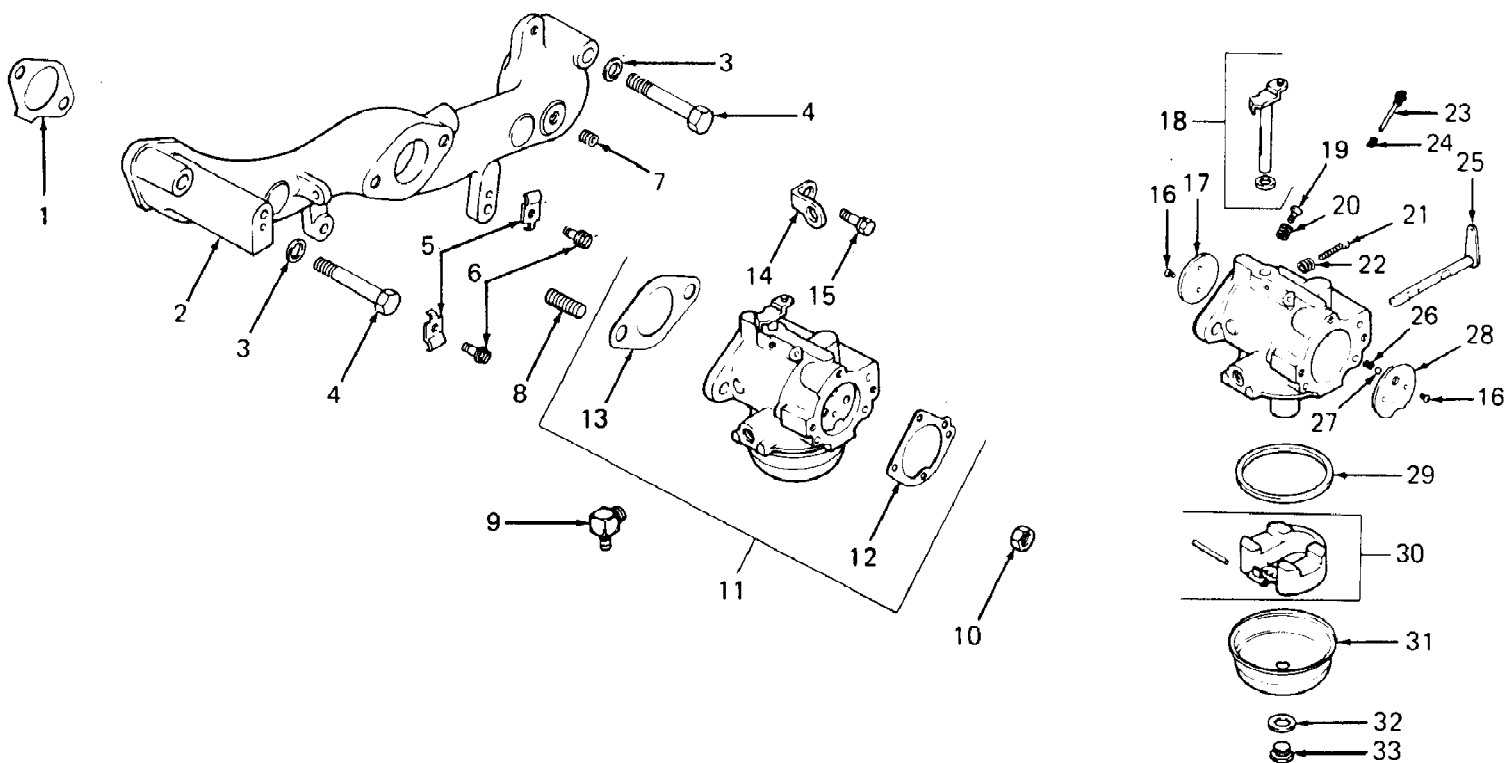
ADJUSTABLE JET CARBURETOR
