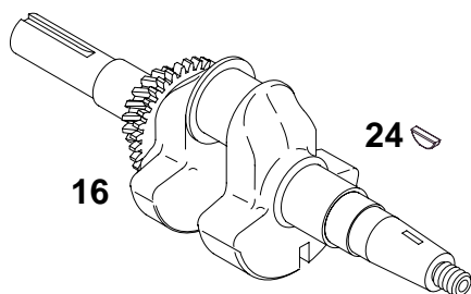
SAE 3/4" KEYWAY
